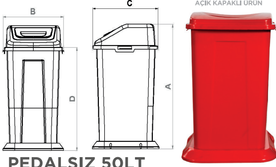
PEDALSIZ 50LT WITHOUT PEDAL
